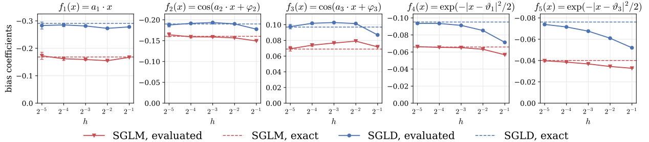
Figure 2: Non-Gaussian noise: the evaluated coefficients (\pi_h(f) - \pi(f))/h of SGLM and (\bar{\pi}_h(f) - \pi(f))/h of SGLD, with error bars of 2 standard errors, and the exact coefficients (6.16), dashed. The vertical axis starts at 0 and is reversed for negative exact coefficients.
