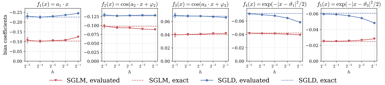
Figure 1: Gaussian noise: the evaluated coefficients (\pi_h(f) - \pi(f))/h of SGLM and (\bar{\pi}_h(f) - \pi(f))/h of SGLD, with error bars of 2 standard errors, and the exact coefficients (6.16), dashed. The vertical axis starts at 0 and is reversed for negative exact coefficients.
