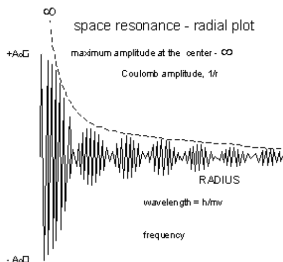
Figure 1.1 (The Line of Infinity): This radial plot contrasts the mathematical absurdity of the Standard Model's 1/r Coulomb potential—which shoots to infinity—with the actual Space Resonance predicted by Milo Wolff. The wave-like amplitude represents the physical reality of the electron, staying finite at the center and resolving the " Infinity Problem " without the need for mathematical fudges like Renormalization.
