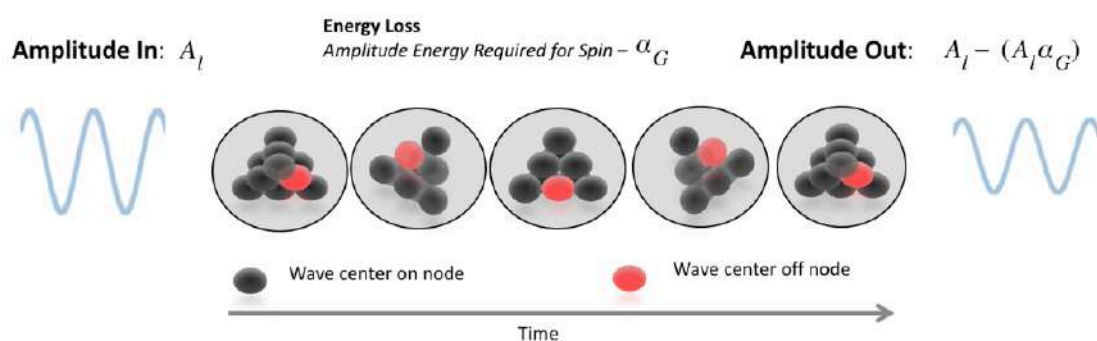
Figure 3a: The Hairdryer Mechanisms of EWT and R.U.T. Compared
