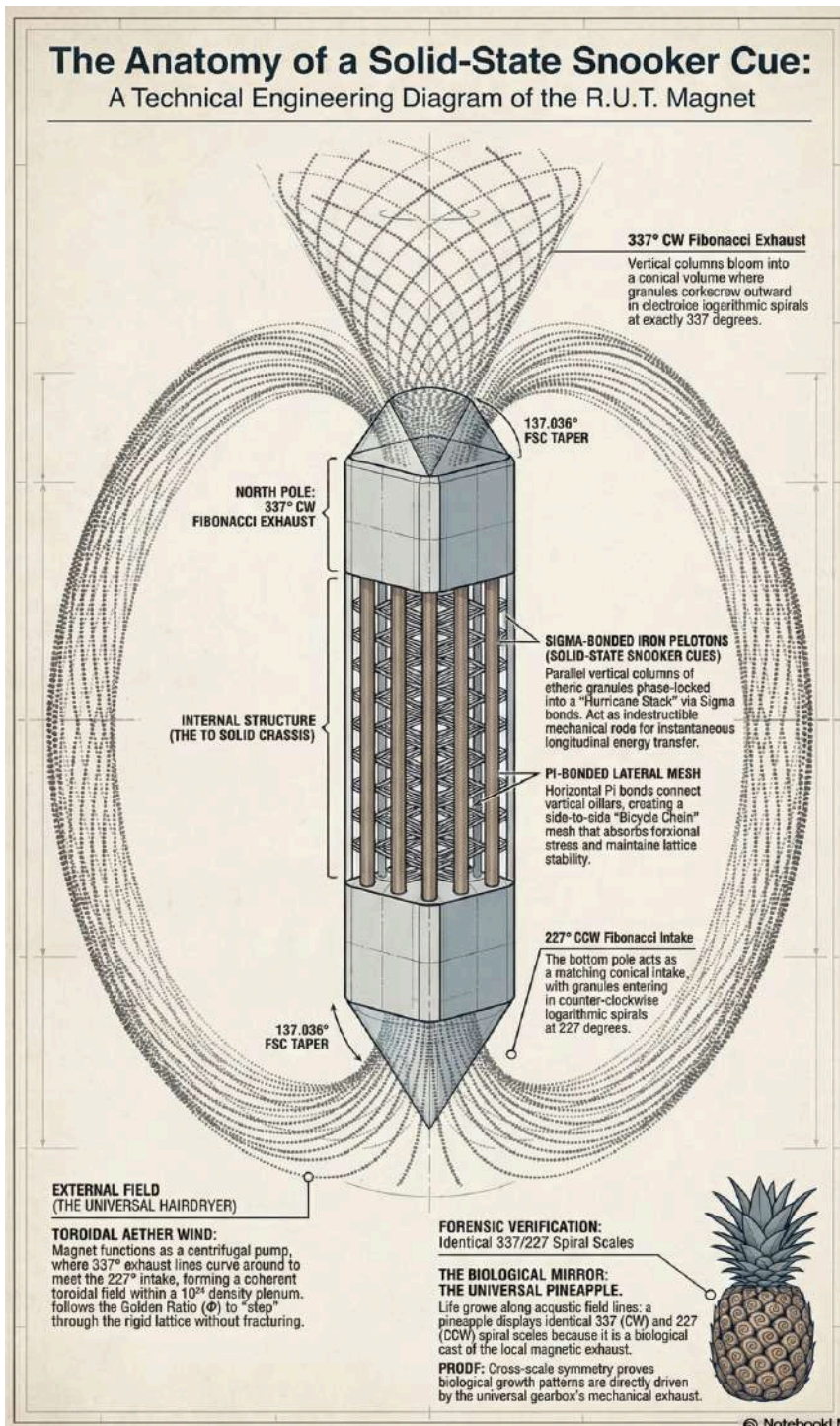
Figure 3c: The Fibonacci Exhaust (Magnetic Blueprint). This technical engineering diagram unmasks the magnet as a Centrifugal Pump . Internal Sigma-bonded Iron Pelotons (Solid-State Snooker Cues) provide the rigid backbone for 1D force transmission. Upon leaving the poles, the Directional Ether Wind follows the 1.35 Expansion Ratio , blooming into 337° Clockwise (North) and 227° Counter-Clockwise (South) spirals.
