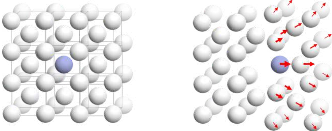
Figure 3.2: The EWT Mechanical Contradiction.
