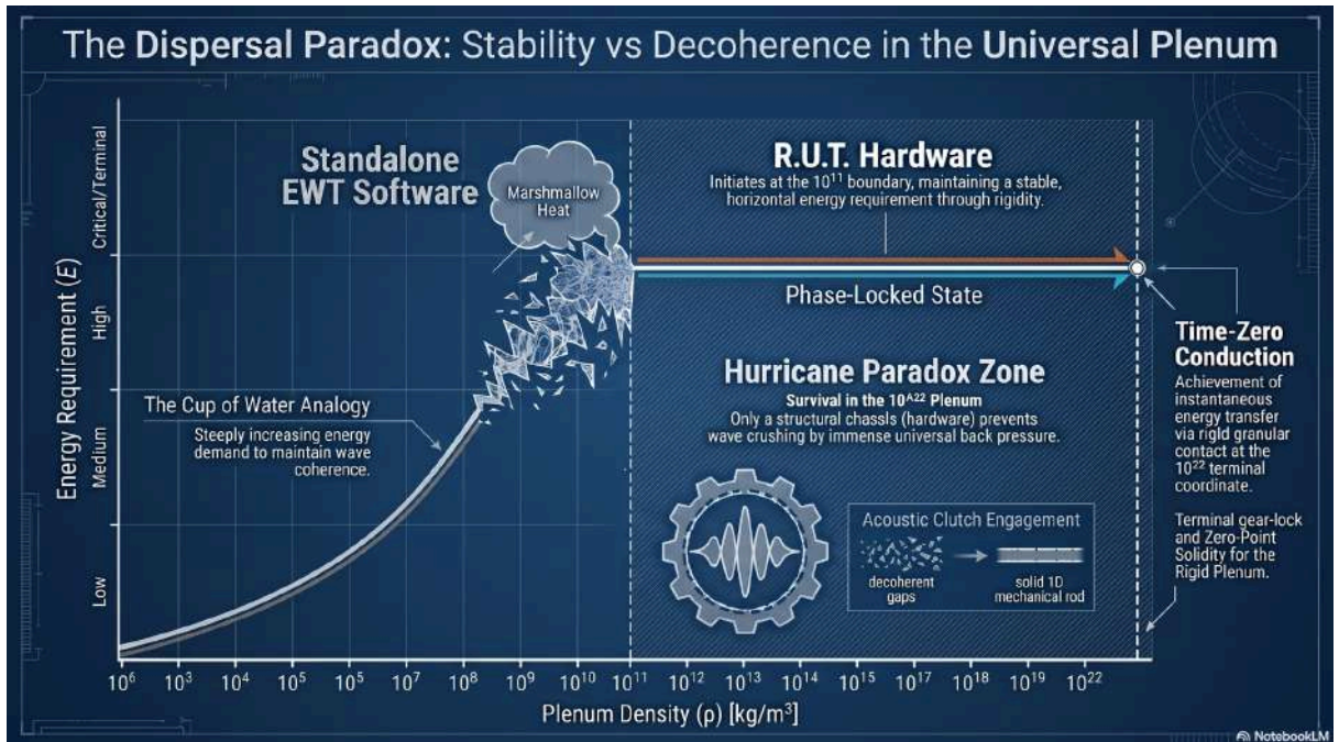
Figure 1.2 (Stability vs. Decoherence) serves as the forensic map for this transition, identifying the 10^{11} kg/m 3 value as the " Geometric Mean Symmetry Break " ( \sqrt{10^{22}}=10^{11} ) that separates mathematical potential from industrial reality.
