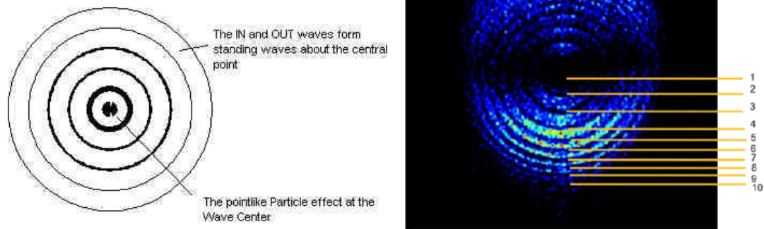
Figure 2.2a: Milo Wolff's Mathematical Prediction (1980s). A theoretical schematic of the Electron as a spherical standing wave, showing the In-waves and Out-waves forming a point-like center.
