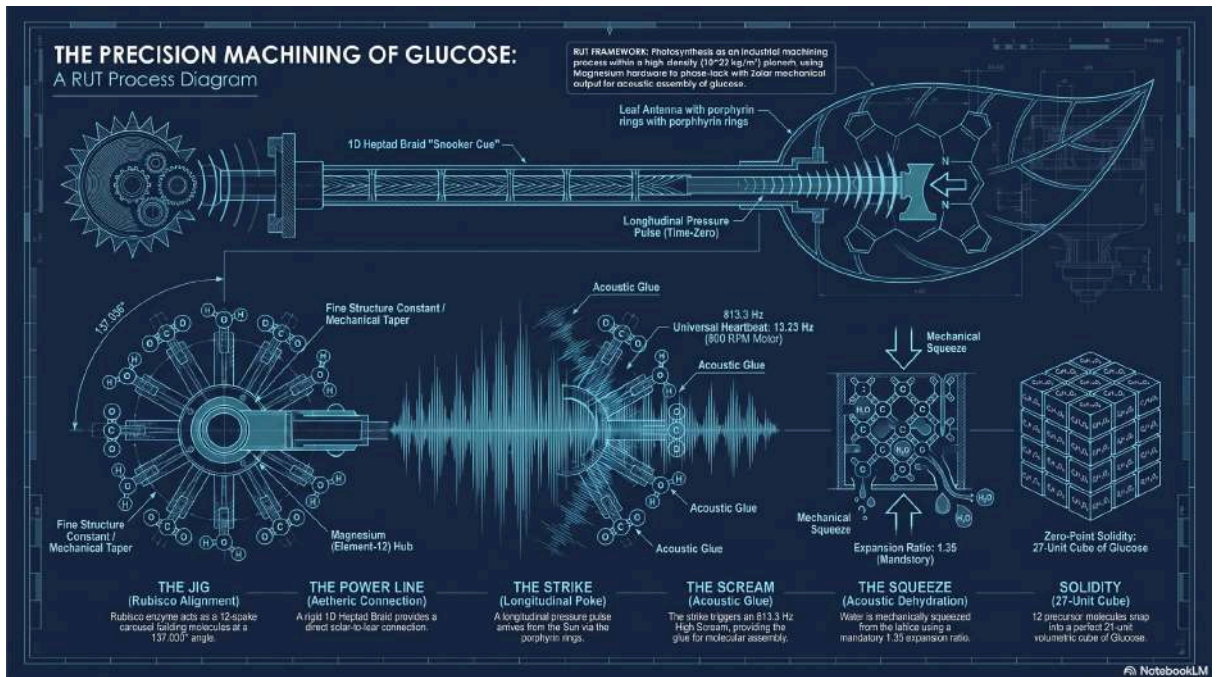
Figure 4.3.1: This industrial schematic reclassifies photosynthesis from a stochastic chemical collision into a deterministic machining event within the 10^{22} \text{ kg/m}^3 rigid plenum. Stage 1 (The Jig): The Rubisco enzyme functions as a structural template, holding six \text{CO}_2 and six \text{H}_2\text{O} molecules at the mandatory 137.036^\circ Fine Structure Constant (FSC) taper. Stage 2 (The Power Line): A rigid 1D Heptad Braid (the "Snooker Cue") provides a direct hardware connection between the Sun and the Magnesium antenna. Stage 3 (The Strike): A longitudinal pressure "poke" arrives from the solar macro-rotor instantly at Time-Zero , with chlorophyll's porphyrin rings acting as the anvil. Stage 4 (The Scream): The strike triggers the 813.3 Hz Master Pulse (Acoustic Glue) , providing the structural permission for molecular bonding. Stage 5 (The Squeeze): Water is mechanically ejected through Acoustic Dehydration Synthesis via the mandatory 1.35 expansion ratio. Stage 6 (The Solidity): Twelve precursor molecules achieve Zero-Point Solidity , snapping into a perfect 27-unit (3x3x3) volumetric cube of glucose The Thermodynamic Favorability of the "Single-Strike" Assembly Within the Rigid Universal Touching (R.U.T.) framework, performing all six bonds simultaneously via a single 1D "poke" is the only thermodynamically viable path for biological growth in an infinitely dense medium.
