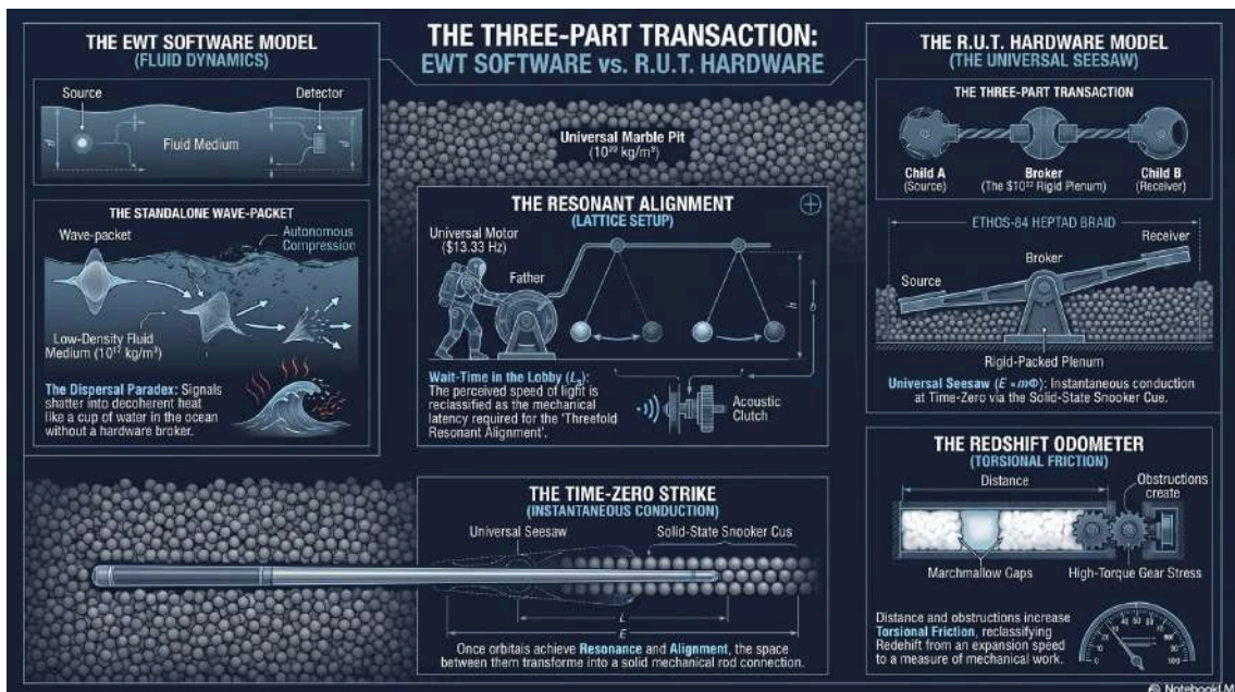
Figure 3.2.1a: The Three-Part Transaction: EWT Software vs. R.U.T. Hardware. This technical infographic illustrates the forensic requirement for the Broker (the 10^{22} kg/m 3 plenum) in energy conduction. While Jeff Yee's EWT (the "Software") successfully identifies the Source and Receiver mechanics, R.U.T. formally validates Milo Wolff's mandate that energy requires a destination "ready" to receive the signal. Panel 1 illustrates the Dispersal Paradox , where a standalone packet shatters like a "cup of water in an ocean" without a hardware broker. Panel 2 illustrates the Universal Seesaw ( E = m\Phi ), where the Ethos-84 Heptad (the 1D Snooker Cue) provides the rigid backbone required for Time-Zero conduction ,. Once the 13.33 Hz motor achieves the Threefold
