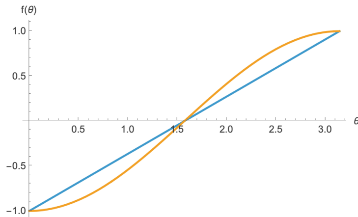
Figure 1: \frac{2}{\pi}\theta - 1 (blue), -\text{Cos}(\theta) (orange)
