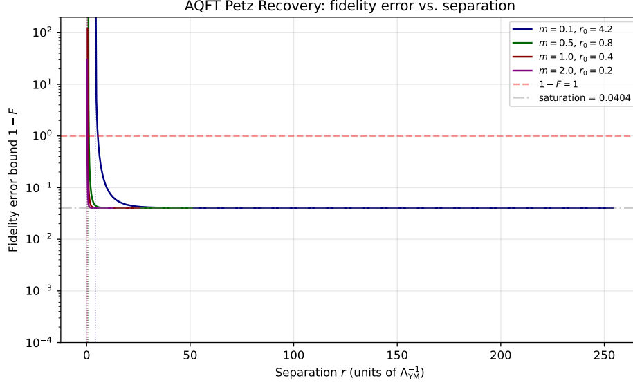
Figure 1: Fidelity error bound 1 - F as a function of spatial separation r for four values of the mass gap m . Vertical dotted lines mark the validity threshold r_0 for each m . The horizontal dashed red line marks 1 - F = 1 ; the gray dot-dashed line marks the saturation value 0.0404. All curves are monotonically decreasing beyond their respective r_0 .
