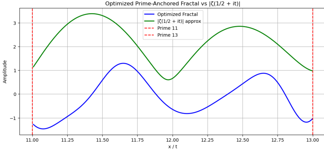
Figure 3: Comparison of the optimized prime-anchored fractal (blue) and the approximate |\zeta(1/2 + it)| (green) between two consecutive primes in this case the interval [11,13] Red dashed lines indicate the prime positions. The local spectral content of the fractal closely matches that of the zeta function.
