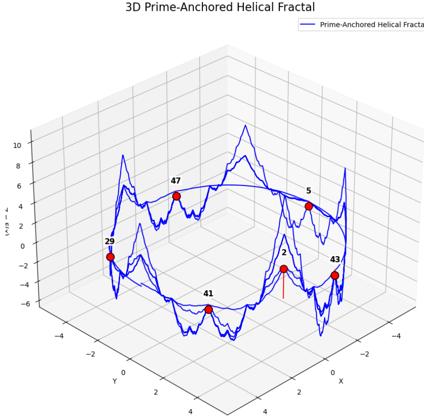
Figure 2: 3D helical prime-anchored fractal. Red markers indicate primes, with labels.
