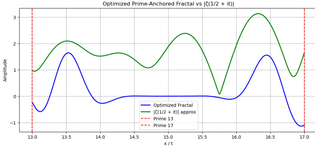
Figure 4: Comparison of the optimized prime-anchored fractal (blue) and the approximate |\zeta(1/2 + it)| (green) between two consecutive primes, in this case the interval [13, 17] . Red dashed lines indicate the prime positions. The local spectral content of the fractal closely matches that of the zeta function.
